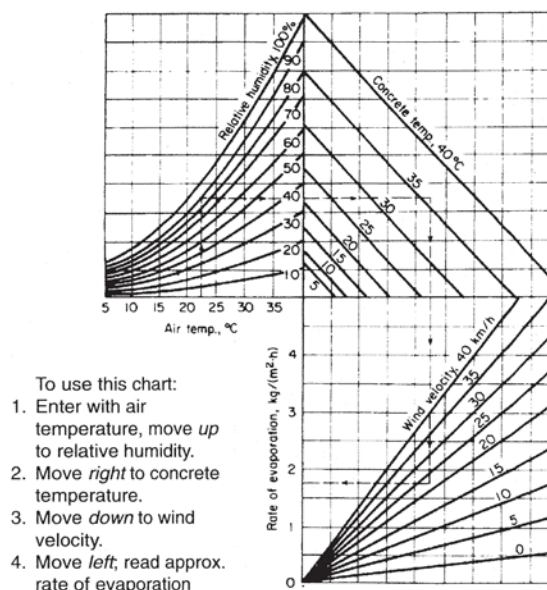
Fig. 12-9. Effect of concrete and air temperatures, relative humidity, and wind velocity on rate of evaporation of surface moisture from concrete. Reference 12-2.
