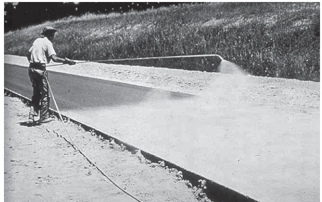
Application of liquid-forming compound with hand sprayer
